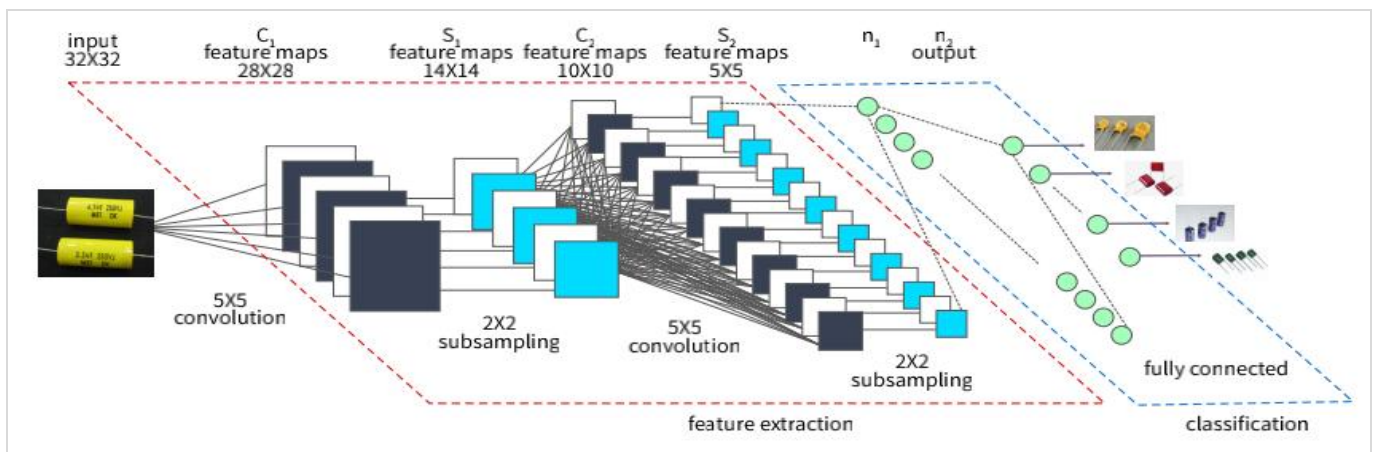
Deep Learning Algorithm
